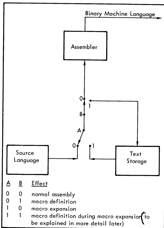
Figure 3. Information Flow During Macro Processing
